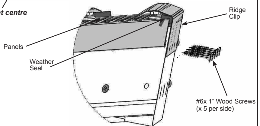
Fig. 10.4 Side View
